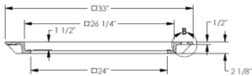
CBCIF - 5426Z FRAME
