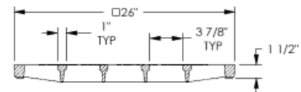
CBBPG - 5426M BIKE PROOF GRATE
